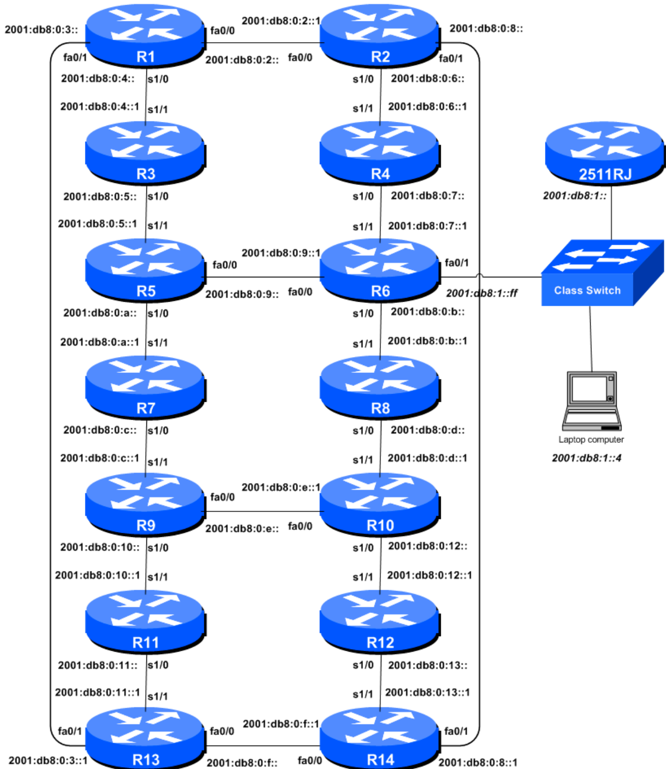
Figure 1 – Addressing scheme for Labs 3 & 4
